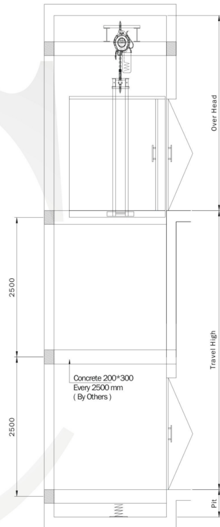
SHAFT SECTION
