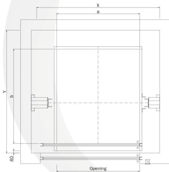
SHAFT PLAN
