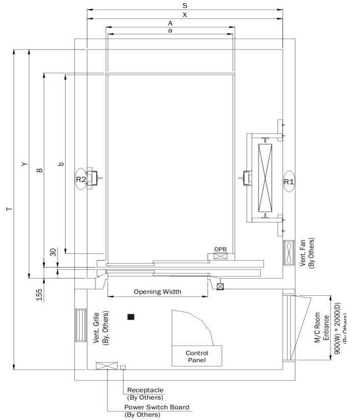
Hoist way Plan
