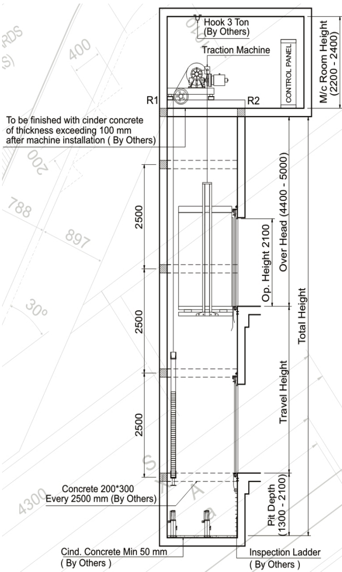
Section Plan
